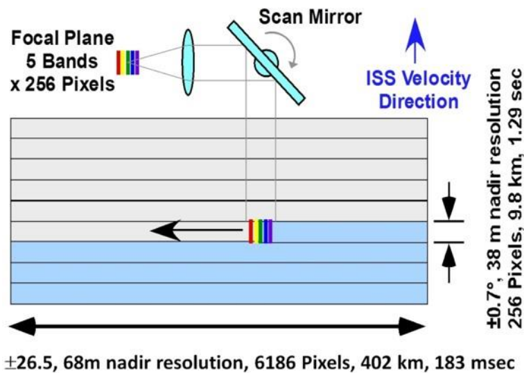
Figure 2.1: ECOSTRESS TIR Scanning Scheme
