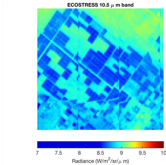
Figure 3.2.1: Illustration of ECOSTRESS Overlap between scans.
