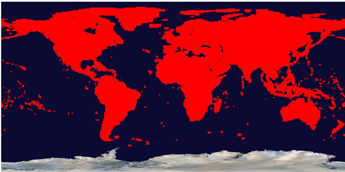
Figure 4: HLS v1.5 covers the global land, including major islands but excluding Antarctica.
