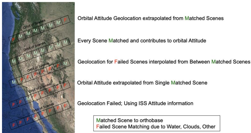
Figure 4.2.1: Orbital Geolocation from Scene Matching
