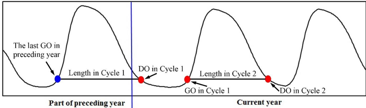
Figure 4. An example of recording metrics related to growing season length if a growing season spans parts of preceding year and current year. Cycle 1 refers to the first data cycle (layer) and Cycle 2 refers to the second one in the product. GO - greenup onset and DO - dormancy onset.
