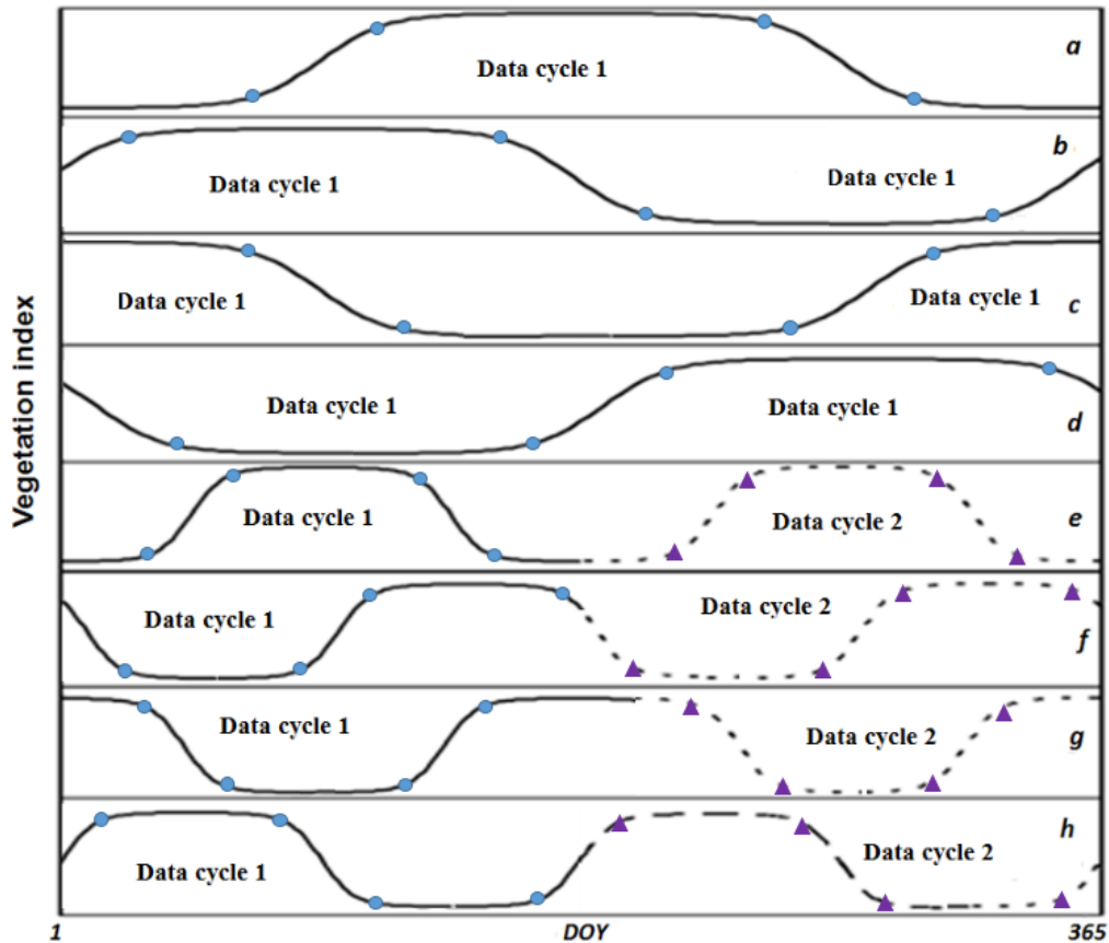
Figure 3. Data cycles recorded in the VIIRS GLSP product during a calendar year. Solid line represents data cycle 1 while dashed line represents data cycle 2. The solid dots are the four phenological dates in the data cycle 1 (first data layer) and solid triangles are the four phenological dates in the data cycle 2 (second data layer).
