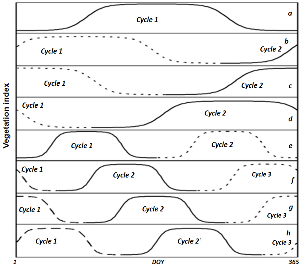
Figure 2. Characteristics of vegetation growing cycles during a 12-month period (current year).
