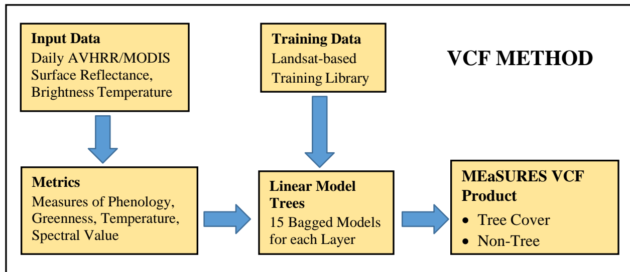
Figure 2. Summary of the MEaSURES VCF method.
