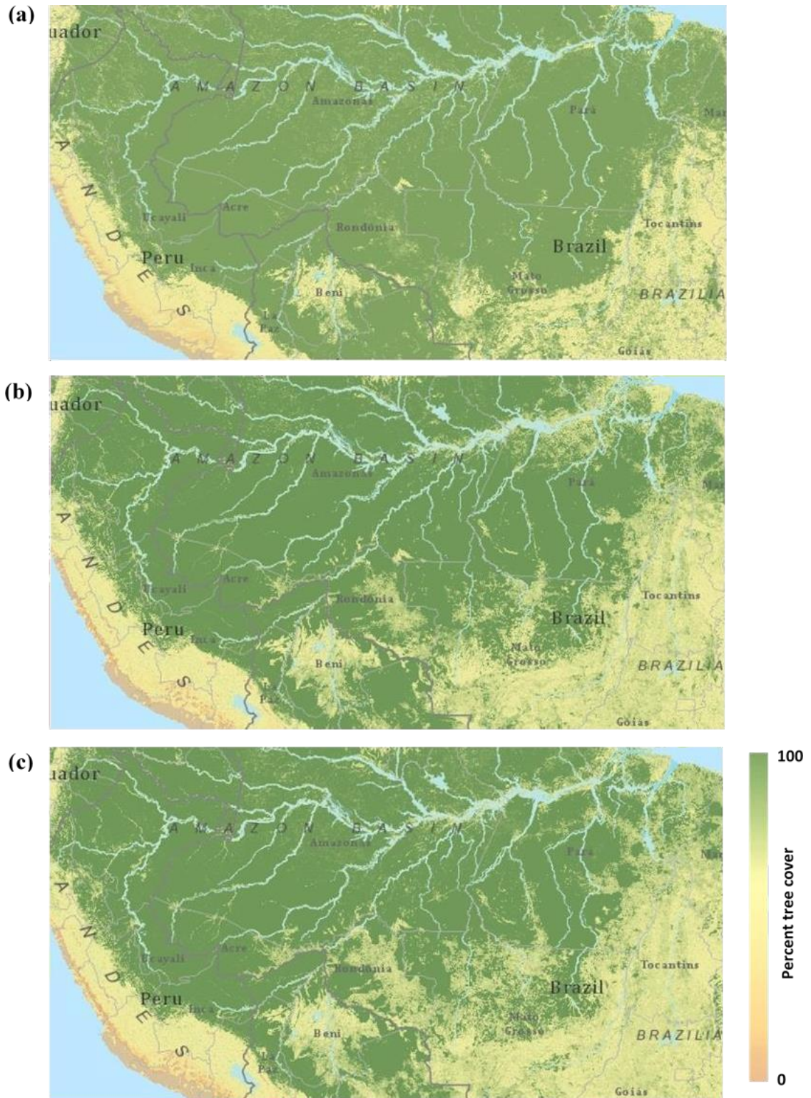
Figure 1. Time series of VCF tree cover for the Amazon Basin from the MEaSUREs VCF ESDR project. (a) 1990, (b) 2000, (c) 2010. Increasing deforestation can be noted in “arc of deforestation” shown in the lower and right sides of the images.
