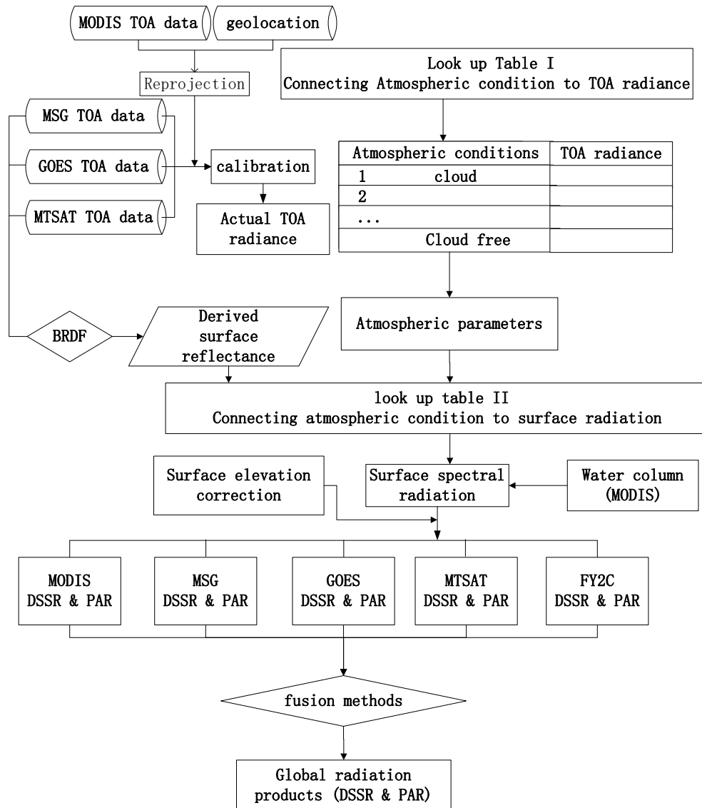
Figure 2. Flowchart to generate global DSR and PAR products from MODIS and geostationary satellite data
