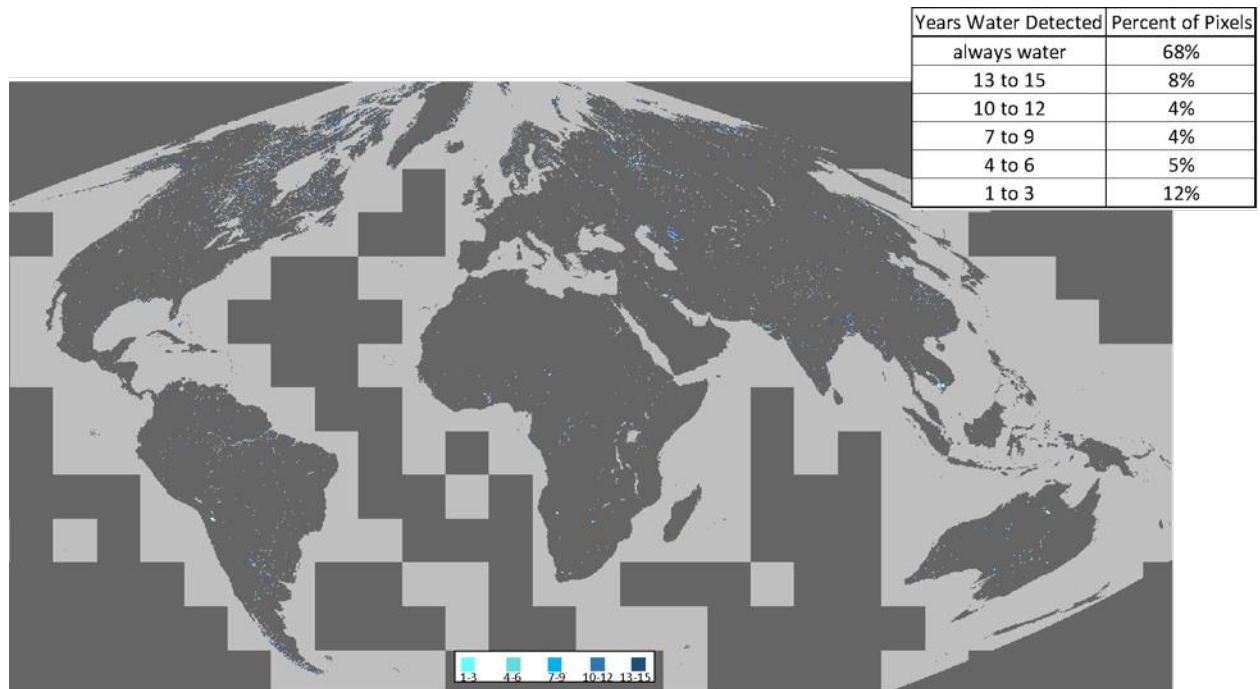
Figure 2 Global map showing the frequency of occurrence of water from all 16 years of MODIS surface water extent. Dark gray is land or no data; light gray is always water; and light blue to dark blue shows an increasing number of years where water was detected.
