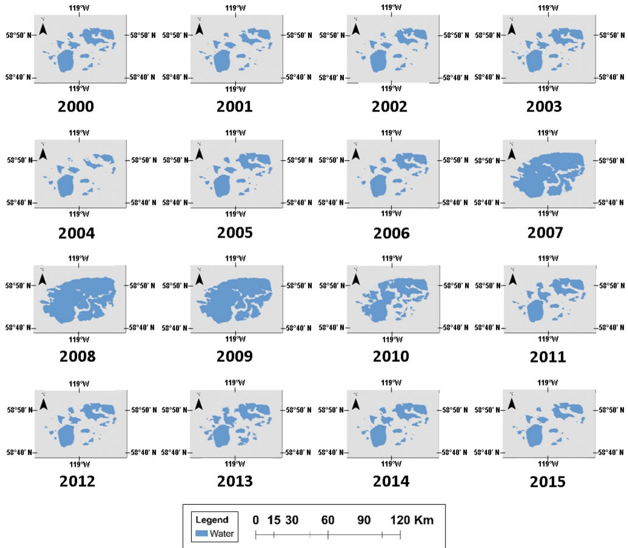
Figure 5 Annual maps of the extent of Hay Lake showing significant inter-annual variability in the lake complex over time.
