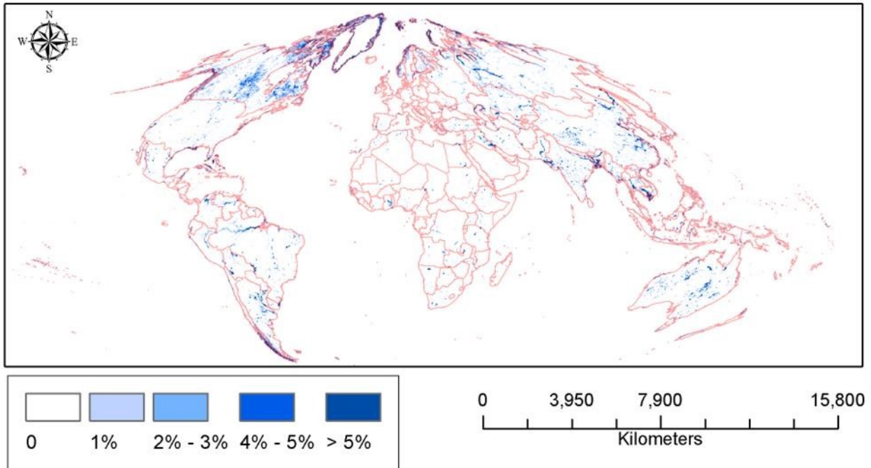
Figure 1 Global map showing the areas where differences between Collection 5 MOD44W and the new Collection 6 MOD44W are most prevalent.
