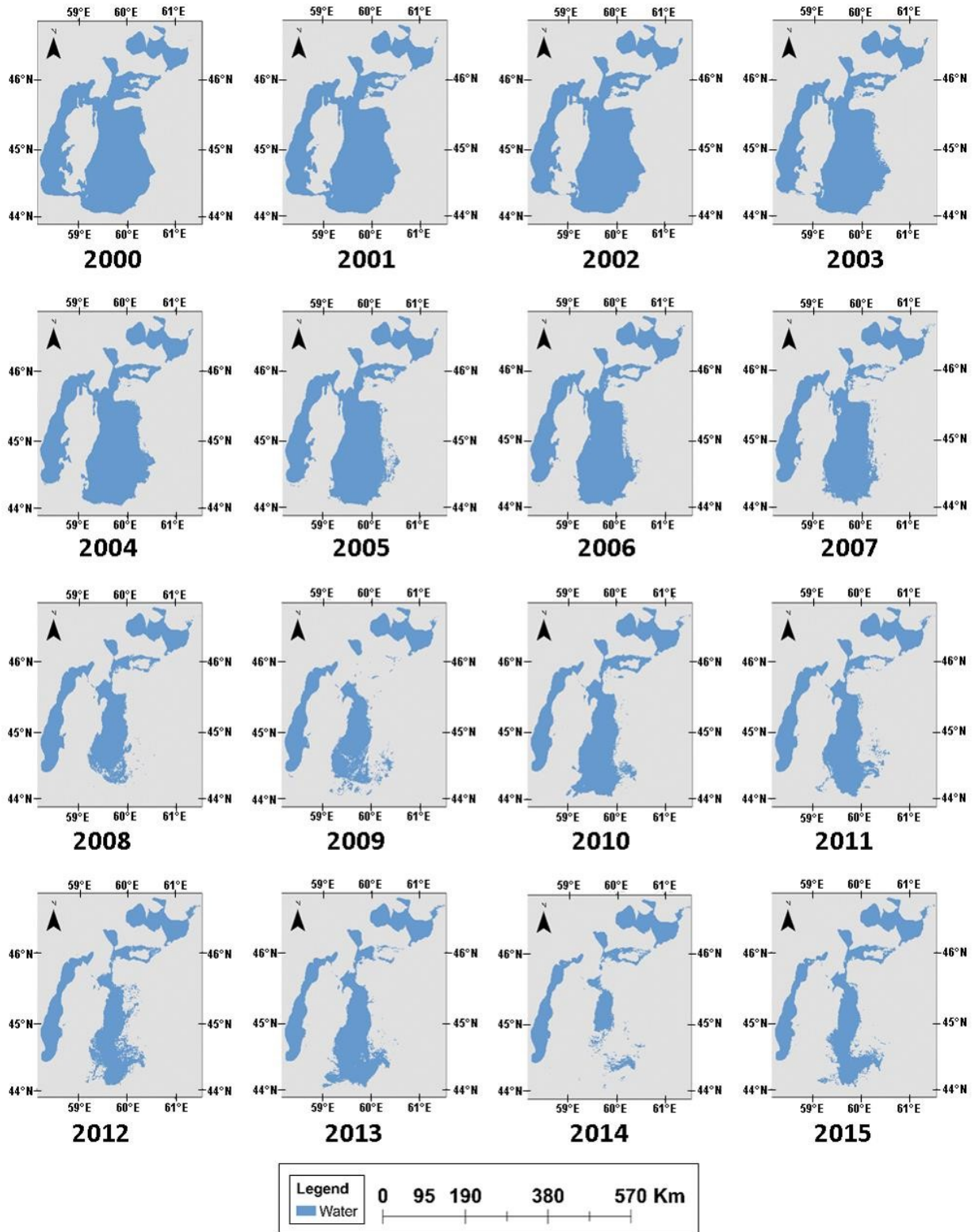
Figure 3 Annual maps of the extent of the Aral sea showing the large scale dessication in just 16 years.
