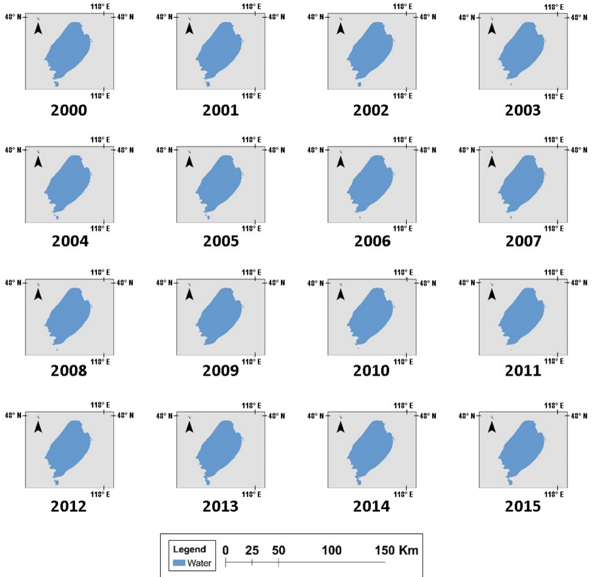
Figure 4 Annual maps of the extent of Lake Bei'er showing it is generally stable through time.
